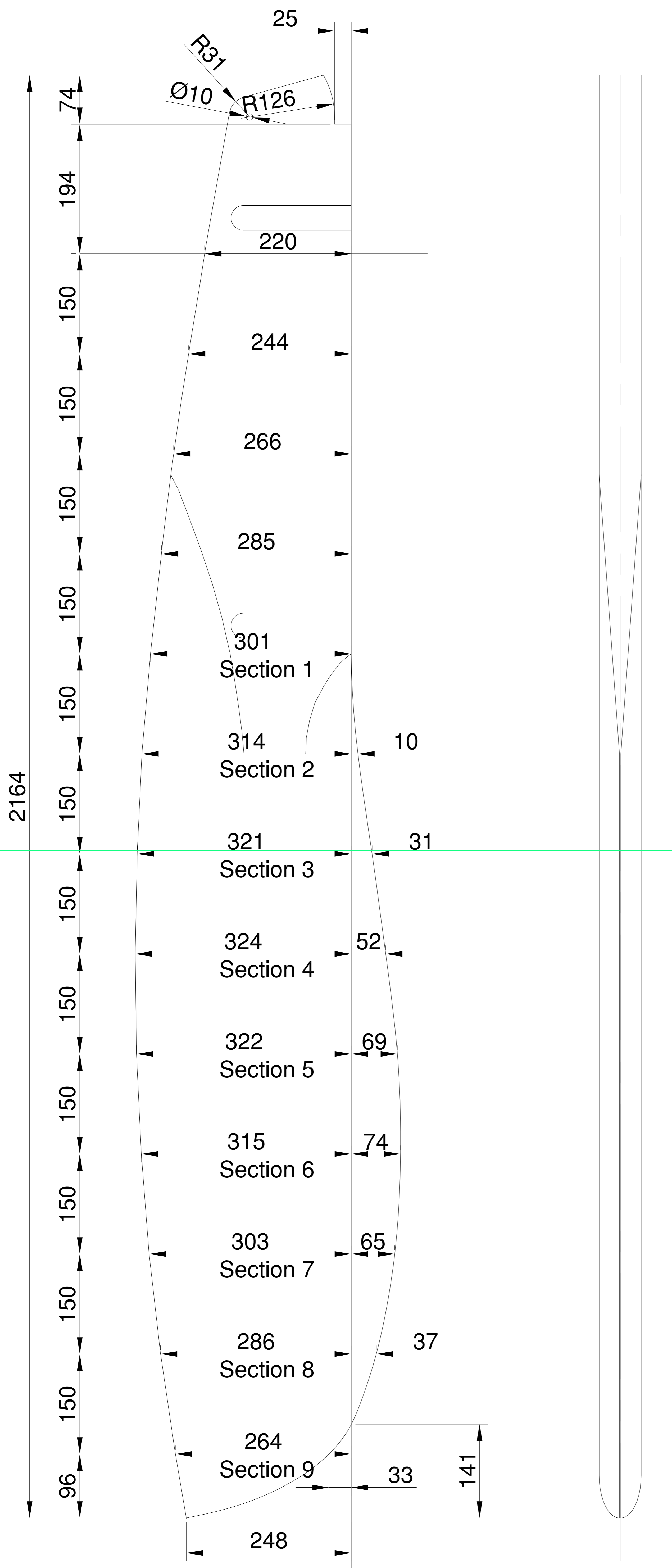
1 IMPALA 28 OOD - Mk2 Rudder Plans
